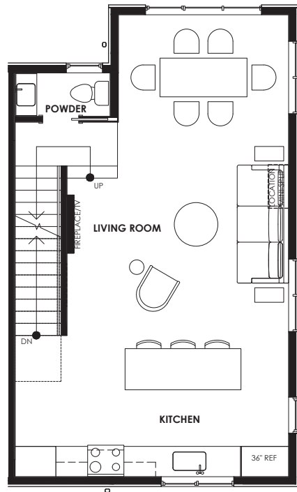
TH 4 - Level 2
