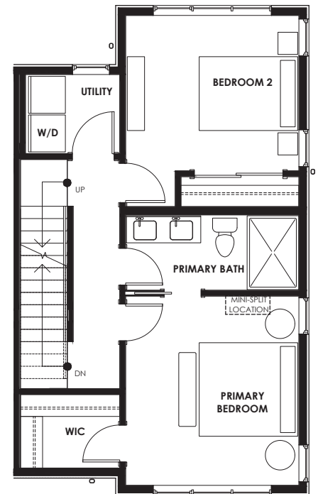
TH 4 - Level 3
